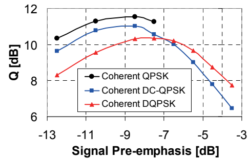
Figure 4: Power pre emphasis sweep for 23 Gbaud single polarization channel at ~1550 nm after 4,200 km distance with coherent QPSK (round symbols), coherent DC-QPSK (square symbols), and coherent DQPSK (triangle symbols).
