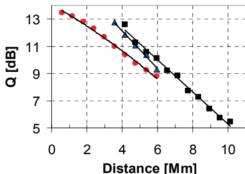
Figure 6: Performance vs. distance for channel at ~1550 nm. Square symbols: 11.5 Gbaud coherent PDM-DC-QPSK; triangles: 23 Gbaud single polarization coherent DC-QPSK; round symbols: 23 Gbaud noncoherent DQPSK.
