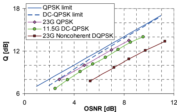
Figure 3: Back-to-back performance (OSNR in 0.4 nm RBW). Theoretical limits for coherent QPSK (solid line) and DC-QPSK (dashed line). Measured QPSK at 23 Gbaud (diamond symbols), DC-QPSK at 11.5 Gbaud dual polarization (round symbols), and noncoherent DQPSK at 23 Gbaud (square symbols).
