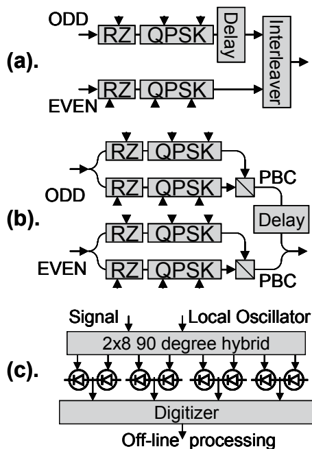
Figure 1: Schematic of single polarization RZ-QPSK transmitter at 23 Gbaud (a), PDM-RZ-QPSK transmitter at 11.5 Gbaud (b), and coherent receiver (c).
