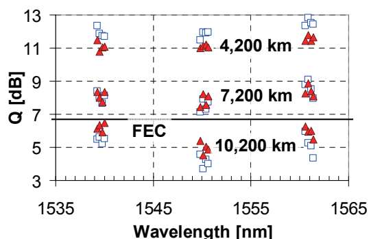
Figure 7: Q-factor after 4,200, 7,200 and 10,200 km distance with coherent DC-QPSK (square symbols) and coherent DQPSK (triangle symbols) for 11.5 Gbaud PDM-QPSK.
