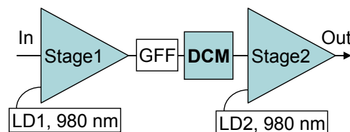
Figure 2: Schematic of the dual-stage EDFA with mid-stage dispersion compensating module DCM.
