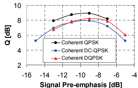
Figure 5: Power pre emphasis sweep for 11.5 Gbaud dual polarization channel after 7,200 km distance with coherent QPSK (round symbols), coherent DC-QPSK (square symbols), and coherent DQPSK (triangle symbols).
